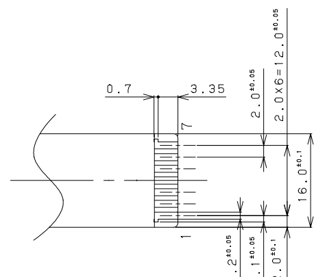
Conductive Face (導通面) FPC-Type Cable
