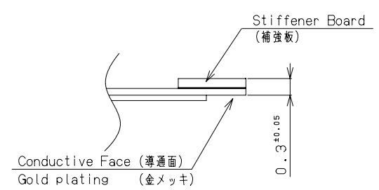
Contact Sectioning View (コネクタ断面図)
