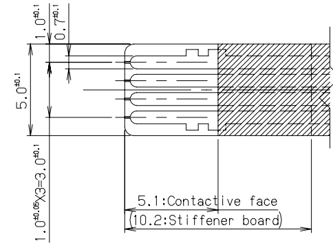
Conductive Face (導通面) FPC-Type Cable
