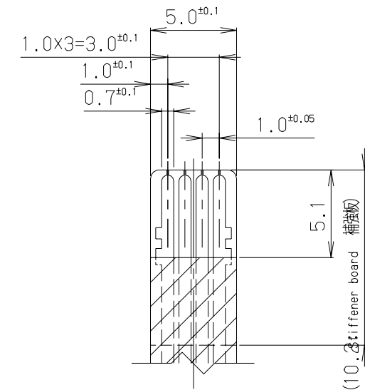
Conductive Face (導通面) FFC-Type Cable
