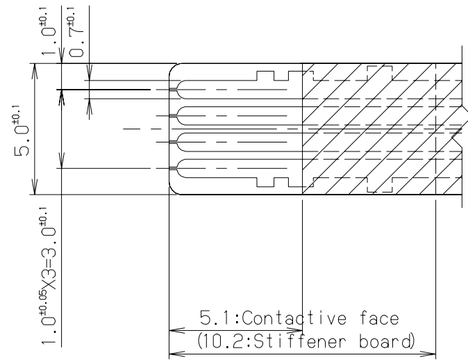
Conductive Face (導通面) FPC-Type Cable
