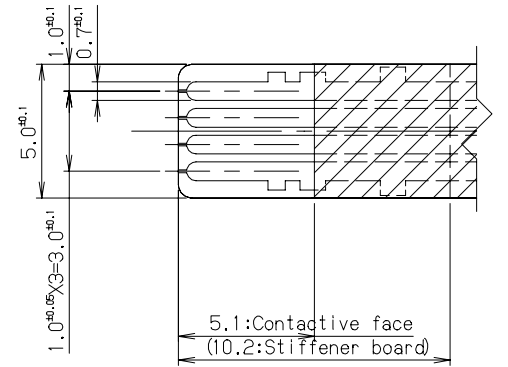
Conductive Face (導通面) FPC-Type Cable
