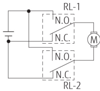
Test circuit
