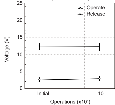
Electrical life (At 30VDC 3A)
