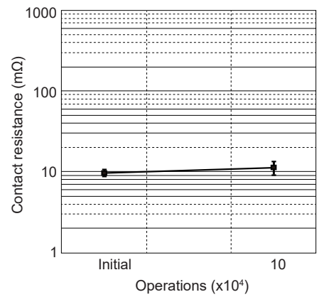
Electrical life (At 250VAC 3A)
