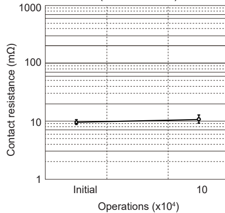
Electrical life (At 30VDC 3A)
