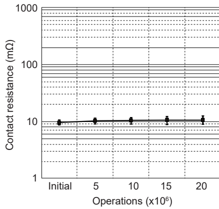
Electrical life (At 250VAC 3A)
