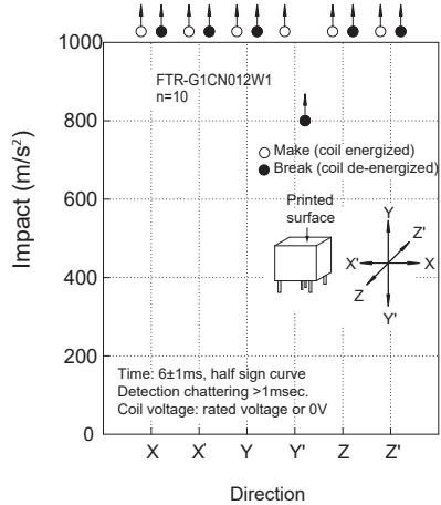
Shock resistance
