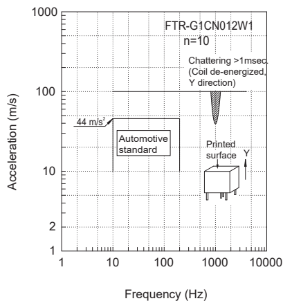
Vibration resistance
