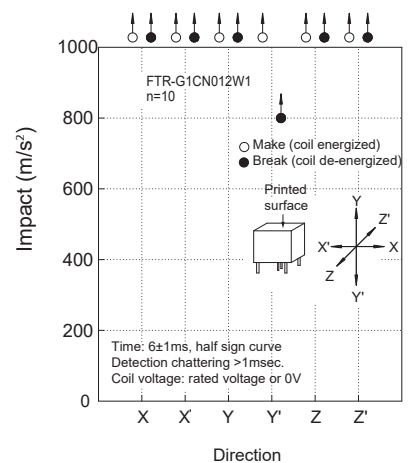
Shock resistance
