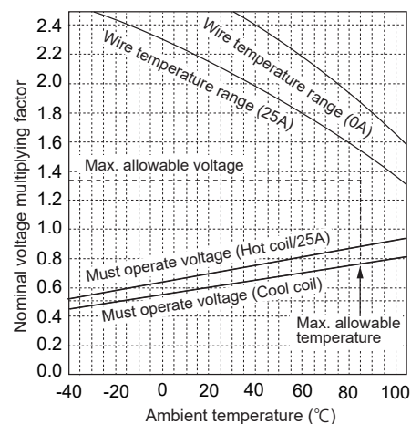
Operating range
