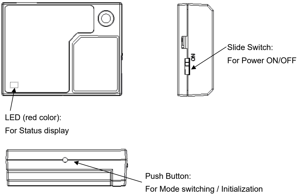
Figure 6-1: Hardware Interface
